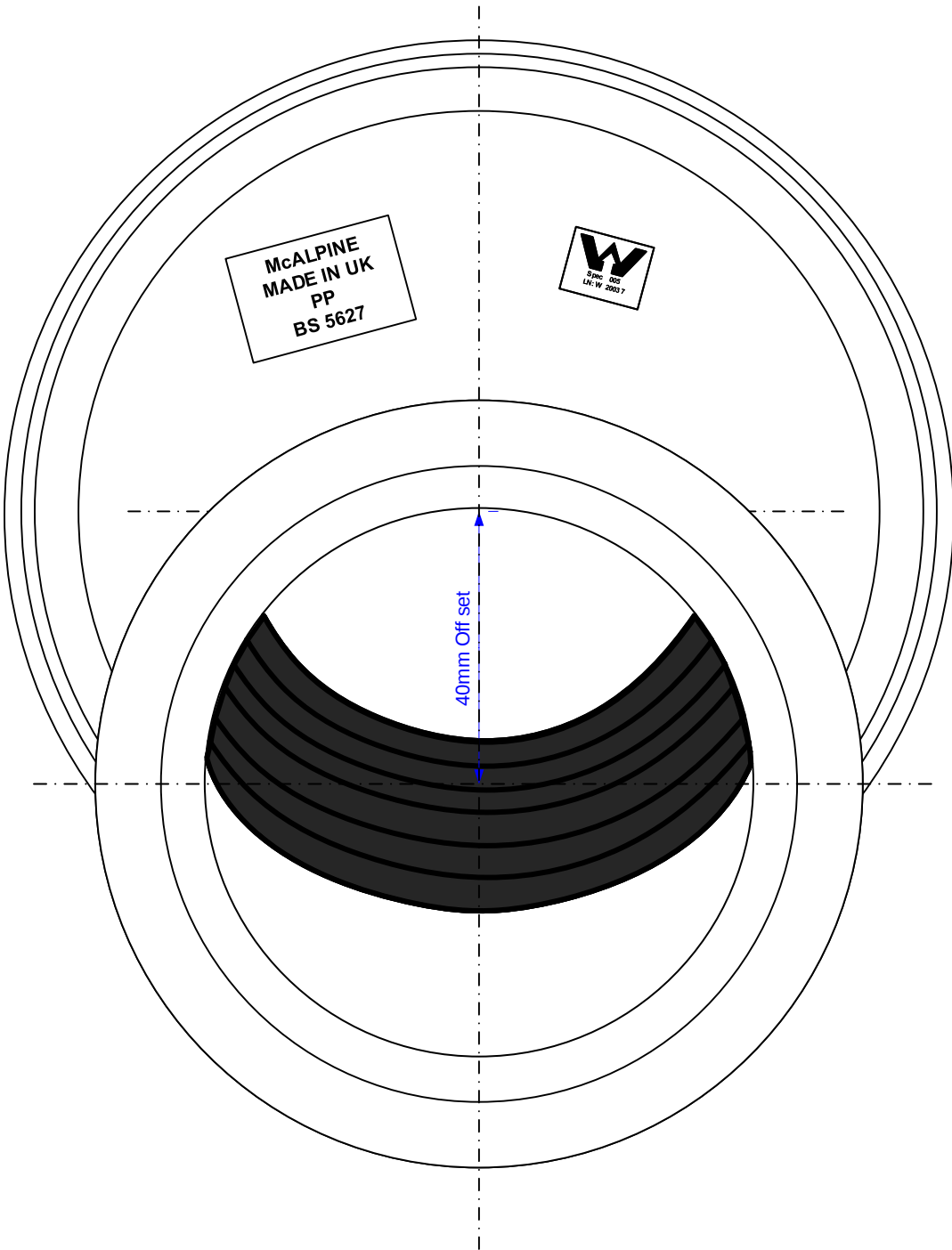
TOP VIEW
