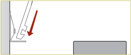
Step 2 As brick wall rises, lower ‘arm’ into ‘anchor’ plate. Reduces injury potential by eliminating jagged edges.
