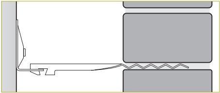
Step 4 Abey Veneer Tremor Ties provide unequalled strength and flexibility against tremors and do not break up mortar under movement.
